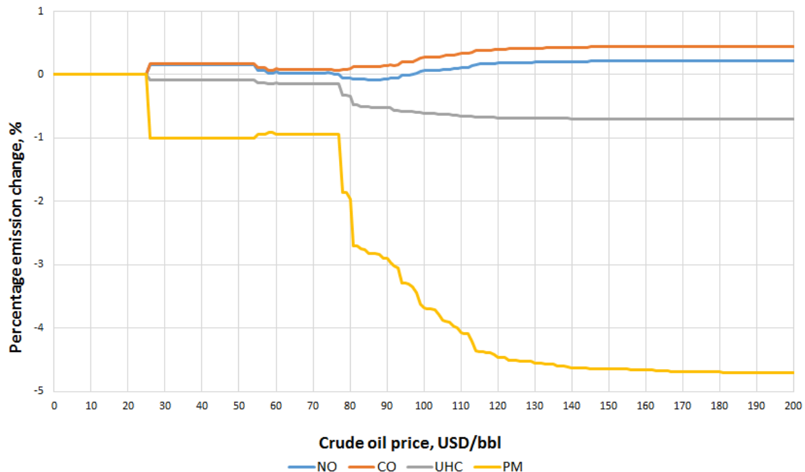
Figure 8: Potential global-scale automotive emission change against crude oil price, as compared to fossil diesel combustion scenario
